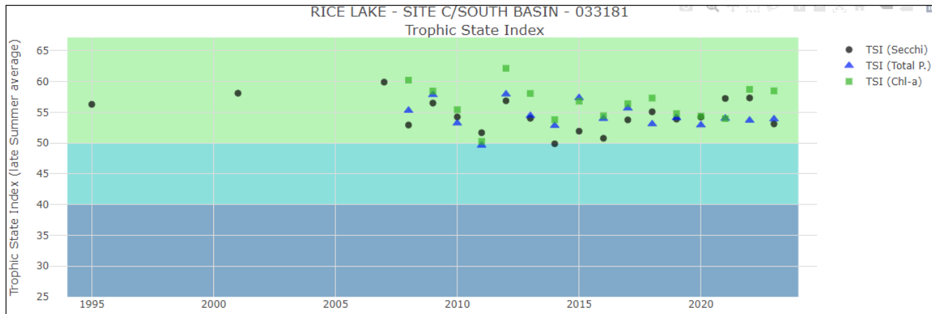
Figure 19: Historical TSI values for water clarity, total phosphorus, and chlorophyll-a at the South Basin in Rice Lake (WEx, 2024)
