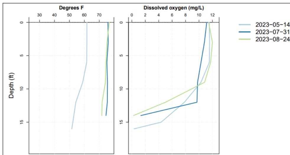
Figure 29: Temperature and DO profiles from the Central Basin of Rice Lake (WEx, 2024)
